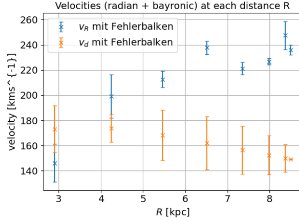
Figure 11: The radial and baryonic velocities at each distance R.
