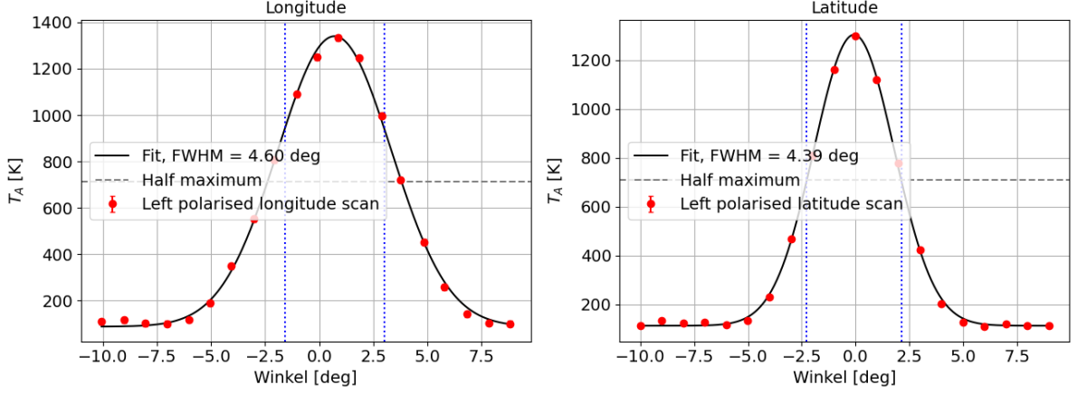
Figure 4: Gaussian fit of the left polarised scan of the longitude (left figure) and latitude (right figure). The FWHM of the fit is marked at 4.6^\circ for the longitude scan and at 4.39^\circ for the latitude scan. The errorbars in both figures are too small to be seen at the scale of the antenna temperature.
