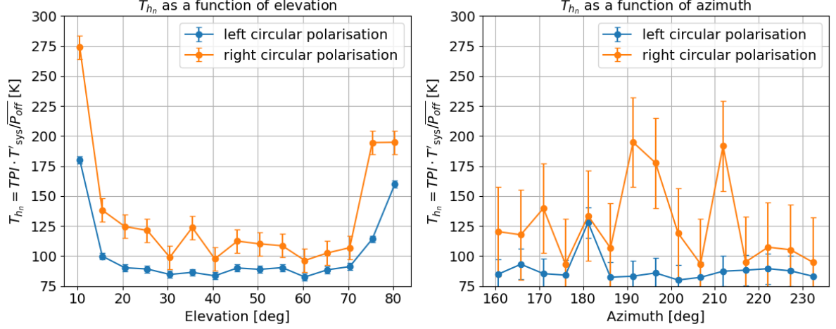
Figure 2: Effective background temperature as a function elevation (left figure) or azimuth (right figure).
