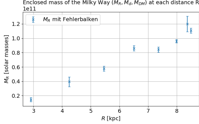
Figure 10: The enclosed mass of the milky way at each distance R.
