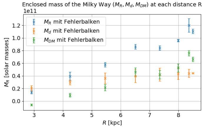
Figure 12: The enclosed mass of the milky way at each distance R broken down for the different mass distributions with M_R being the total enclosed mass, M_d being the enclosed baryonic mass and M_{DM} being the enclosed mass of the dark matter.
