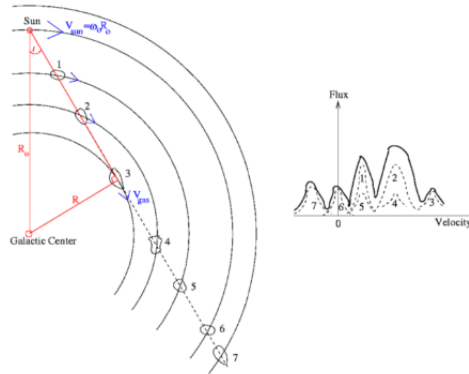
Figure 1: A schematic representation of the rotation of H1 clouds around the galactic centre together with the resulting line profile to the right [1].
