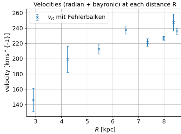
Figure 9: The radial velocity at each distance R .
